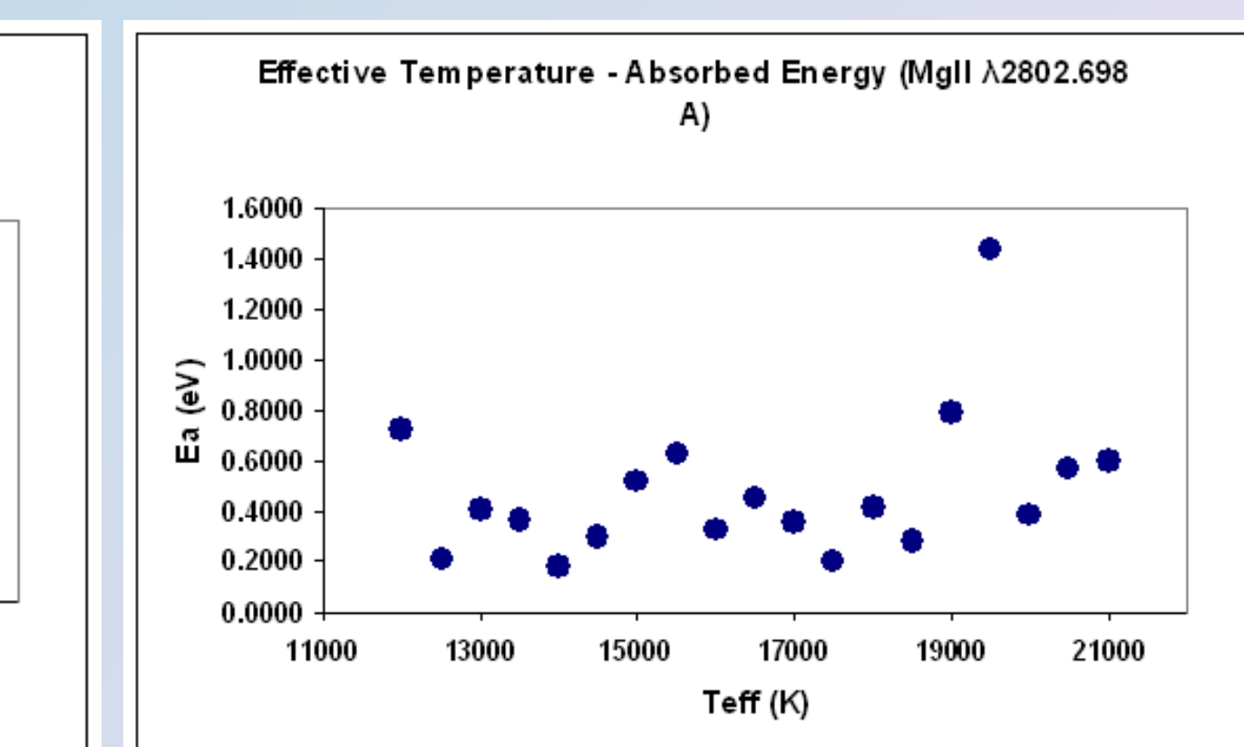
Figure 6. Variation of the absorbed energy ( E_a in eV) of the Mg II resonance line \lambda 2795.523 Å (left) and \lambda 2802.698 Å (right) for the independent density regions of matter which create the 1 or 2 satellite components, as a function of the effective temperature. We note the same variation of the absorbed energy and the FWHM. (see Fig. 5).
