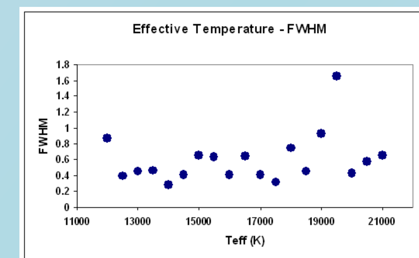
Figure 5. Variation of the Full Width at Half Maximum (FWHM) of the Mg II resonance lines ( \lambda\lambda 2795.523, 2802.698 Å) for the independent density regions of matter which create the 1 or 2 SACs, as a function of the effective temperature. We detected values between 0.2 and 1.6 Å.
