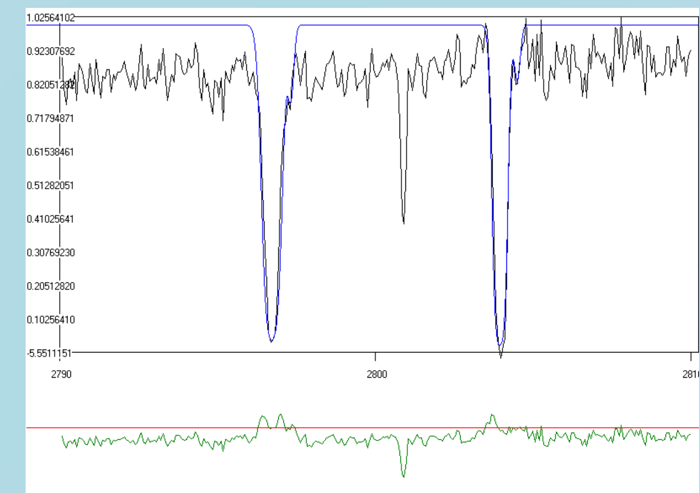
Figure 1: The Mg II \lambda\lambda 2795.523, 2802.698 Å resonance lines in the spectrum of HD 52721. Each of Mg II spectral lines consists of two SACs. The graph below the profile indicates the difference between the fit and the real spectral line.
