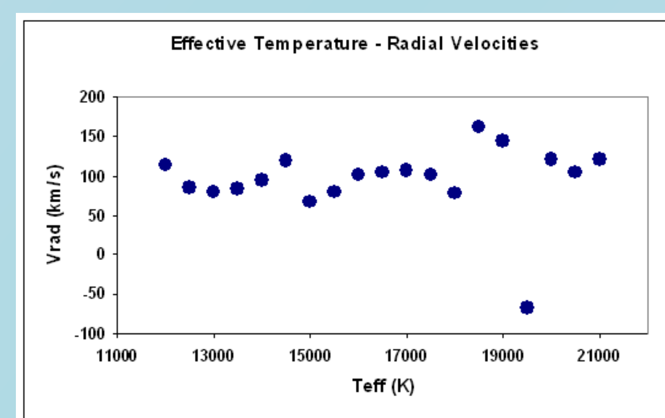
Figure 3. Variation of the radial velocities of the Mg II resonance lines ( \lambda\lambda 2795.523, 2802.698 Å) for the independent density regions of matter which create the 1 or 2 SACs, as a function of the effective temperature. We detected values between 50 and 150 km/s, except in the case of the star HD 45910 where we detected a Mg II density region with radial velocity of about -70 km/s. This case was checked very carefully.
