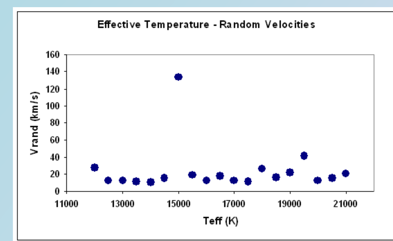
Figure 4. Variation of the random velocities of the Mg II resonance lines ( \lambda\lambda 2795.523, 2802.698 Å) for the independent density regions of matter which create the 1 or 2 SACs, as a function of the effective temperature. We detected values between 10 and 40 km/s, except in the case of the star HD 217050, where the calculated value of the random velocity is about 140 km/s.
