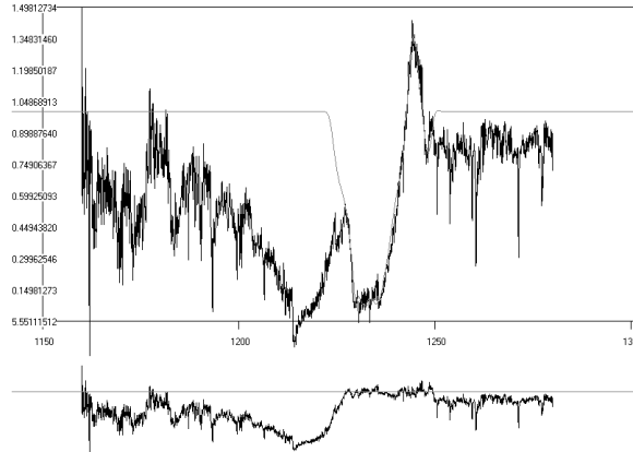
Figure 2: The N V \lambda\lambda 1238.821, 1242.804 Å resonance lines the spectrum SWP18941 of HD 24912. Each of N V spectral lines consists of three SACs.
