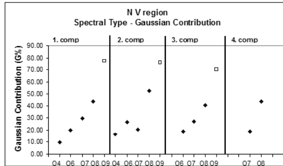
Figure 4: Variation of the mean Gaussian contribution to the line broadening of the N V resonance lines ( \lambda\lambda 1238.821, 1242.804 Å) for the independent density regions of matter which create the 1, 2, 3 and 4 SACs as a function of the spectral subtype. With □ we note the high values of the Gaussian contribution which correspond to the stars where the main reason for the line broadening is the random motions of the ions
