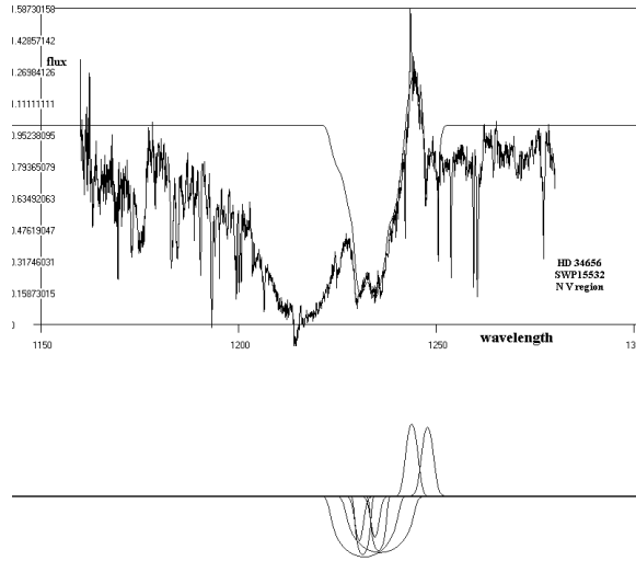
Figure 1: The N V \lambda\lambda 1238.821, 1242.804 Å resonance lines in the spectrum SWP 15532 of HD 34656. Each of N V spectral lines consists of 3 SACs and one emission component. The graph below the fit indicates the components which construct the complex structure of the line above.
