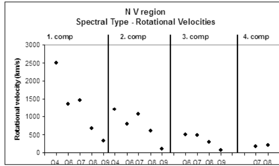
Figure 3: Variation of the rotational velocities' mean values of the N V resonance lines ( \lambda\lambda 1238.821, 1242.804 Å) for the independent density regions of matter which create the 1, 2, 3 and 4 SACs as a function of the spectral subtype.
