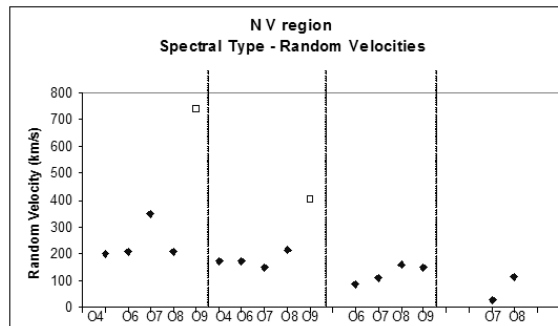
Figure 5: Variation of the mean random velocities of the ions of the N V resonance lines ( \lambda\lambda 1238.821, 1242.804 Å) for the independent density regions of matter which create the 1, 2, 3 and 4 SACs as a function of the spectral subtype. With □ we note the values of the random velocities which correspond to the stars where the main reason for the line broadening is the random motions of the ions
